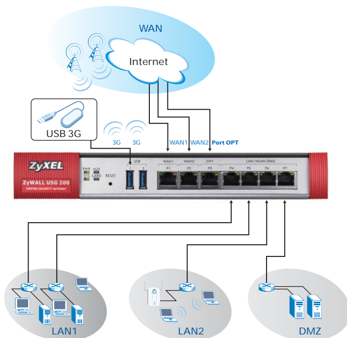
Panneau frontal ZyWALL USG 200
